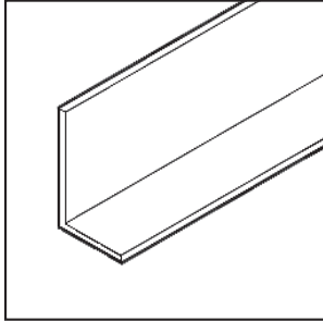
RR-104 END RUN ANGLE Height: 1-1/4" (32mm) Width: 3/4" (19mm) Length: 12'-6" (3810mm)
