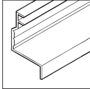
RR-121 MALE ANGLE Height: 2" (51mm) Width: 1-3/8" (35mm) Length: 12'-6" (3810mm)
